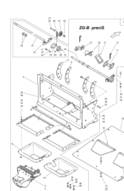
ETB-013140, M-Box ZG-B "preciS"
